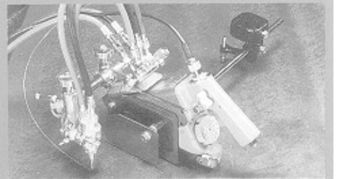
Circular cutting attachment (shown in photograph) Radius 50-550mm (2-22") : S/N60033353 Straight rail 1.8m (12") units: S/N BBA18301
